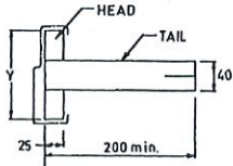
4A Fixing Lug (Holdfast) (Required for Masonry)
